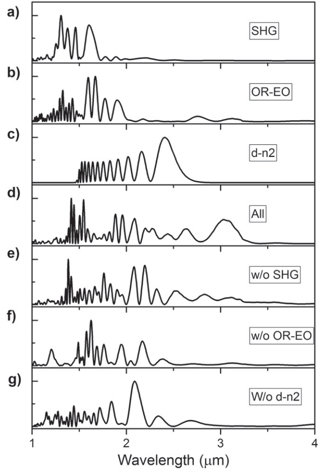
Figure 5. Simulations indicate that mismatched SHG, electro-optical modulation due to optical rectification (OR-EO) and delayed nonlinear refraction (d-n2) contribute to the spectral broadening. (a)–(c) Single process do not mimic the experimental spectrum. (d) Large broadening and redshift similar to the experiment are observed when all the three processes are taken into account. (e)–(g) If one of the nonlinear mechanisms is omitted the agreement with the experimental data becomes worse. The simulations are carried out for a plane wave pump of fluence of 13.5 \text{ mJ cm}^{-2} .
