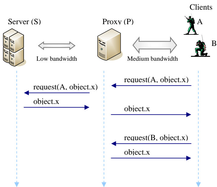
Figure 4: Caching
