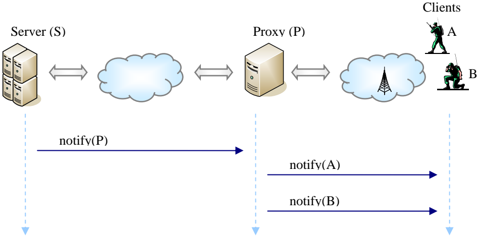
Figure 2: Notification via proxy, unicast
